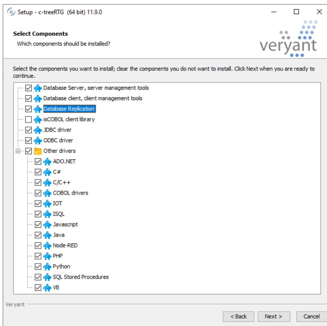
Figure 17. c-treeRTG 11.9 setup
