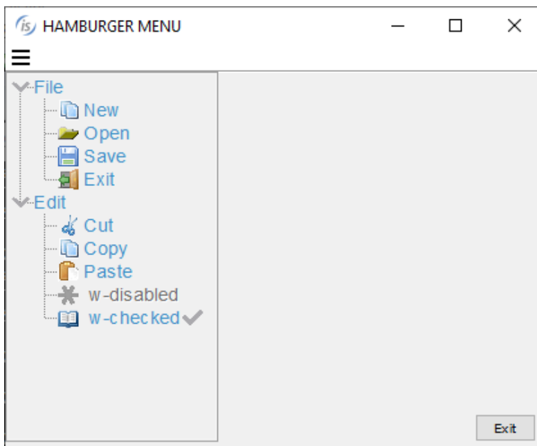
Figure 9. Hamburger menu
