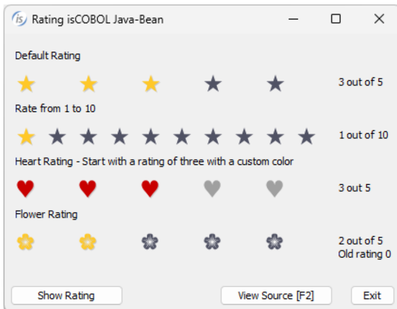
Figure 5. Rating bean.
