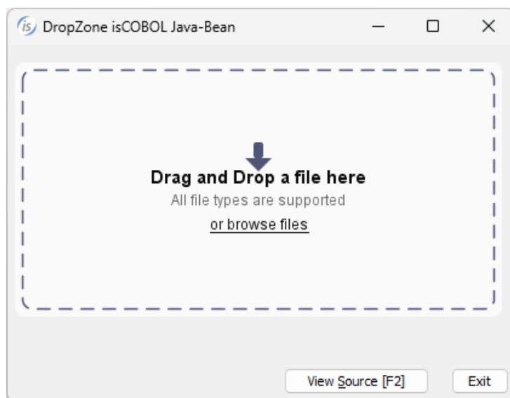
Figure 4. DropZone bean.
